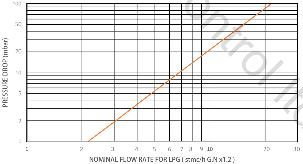
DIAGRAM FLOW RATE: 32051 - 1/2" FOR LPG
