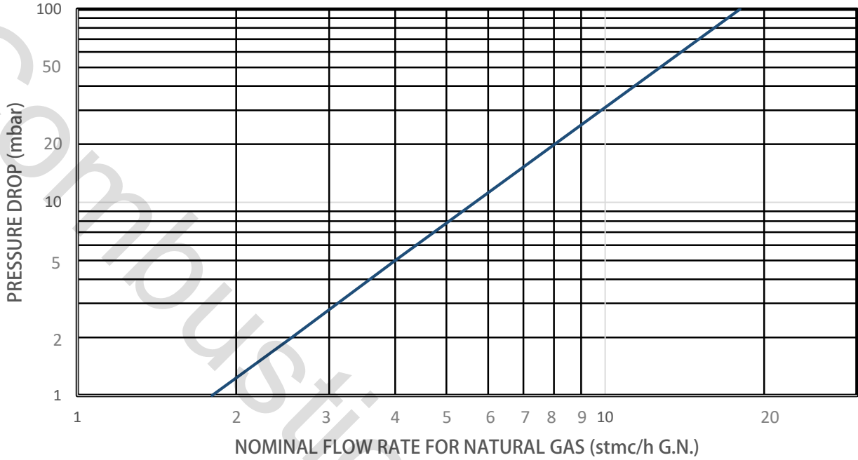
DIAGRAM FLOW RATE: 32051 - 1/2" FOR NATURAL GAS
