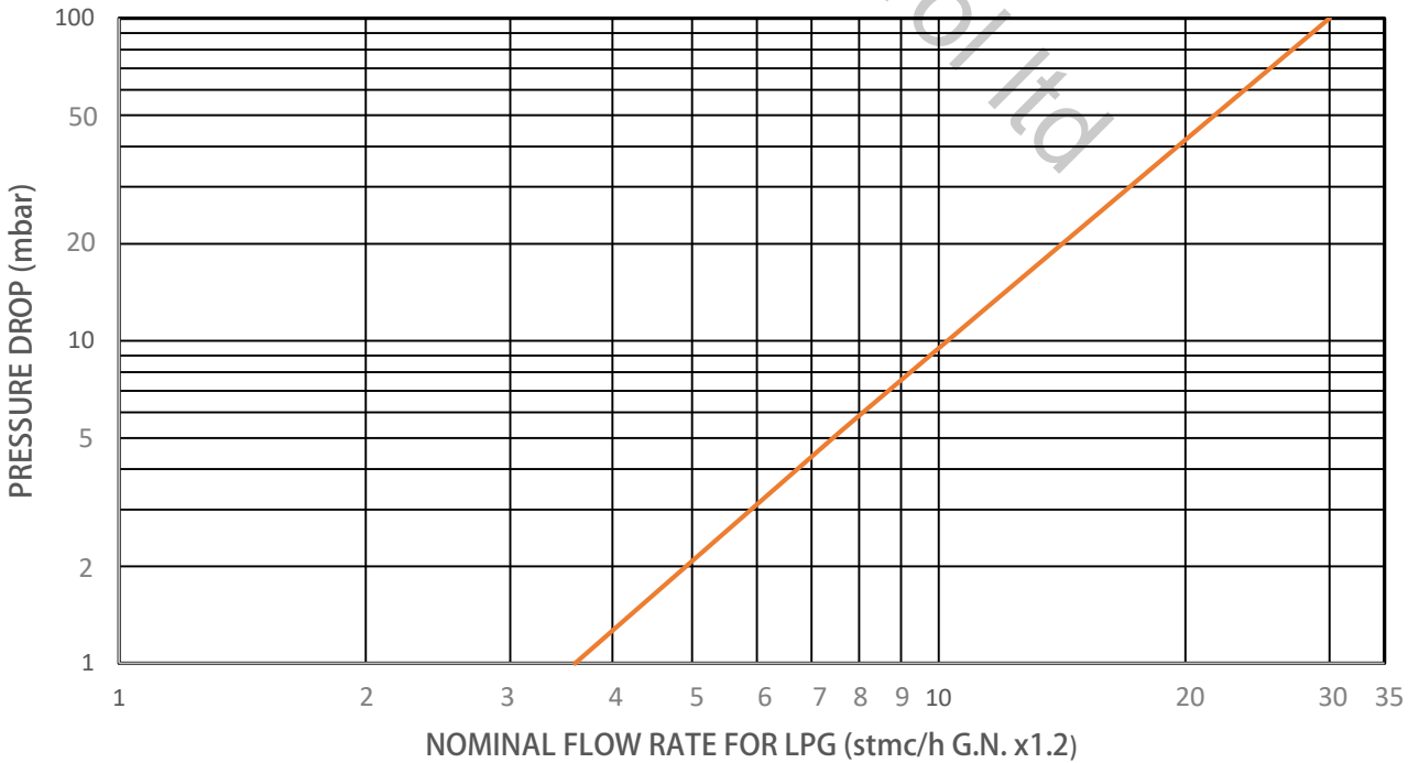
DIAGRAM FLOW RATE: 32052 - 3/4" FOR LPG
