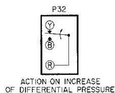
Fig. 3 — Contact action on the P32 Switch.
